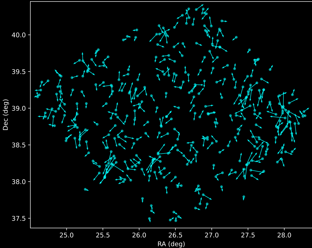
APOGEE DR17 Noise Stream Proper Motion Vectors (n=351)
