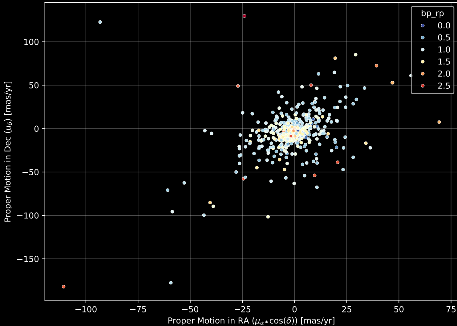
APOGEE DR17 Field: [K18_070+14] Proper Motion Diagram (n= 652)
