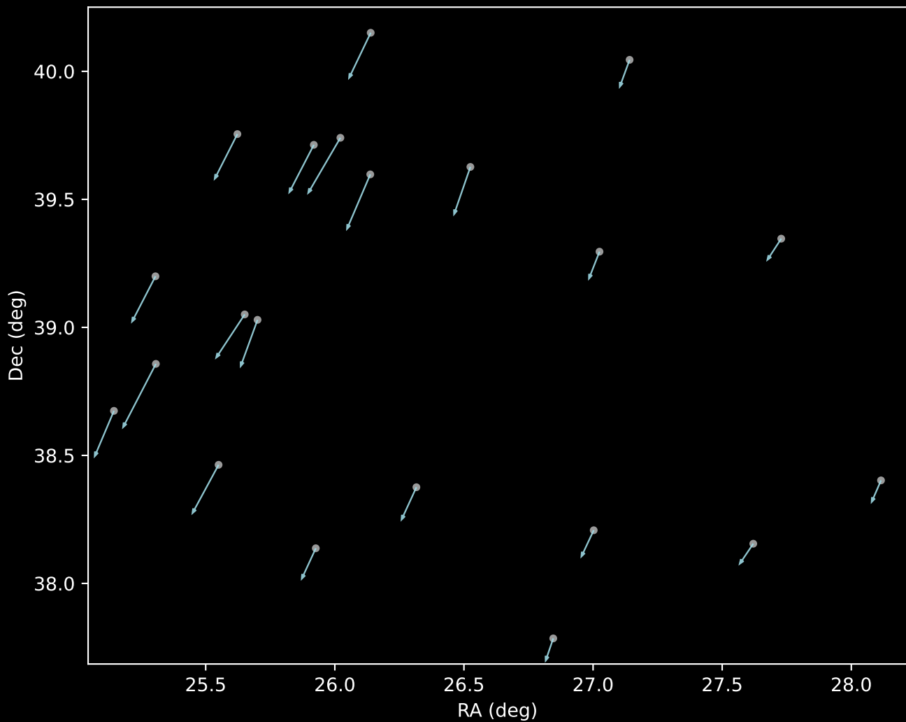
APOGEE DR17 Cluster 19 Proper Motion Vectors (n=21)
