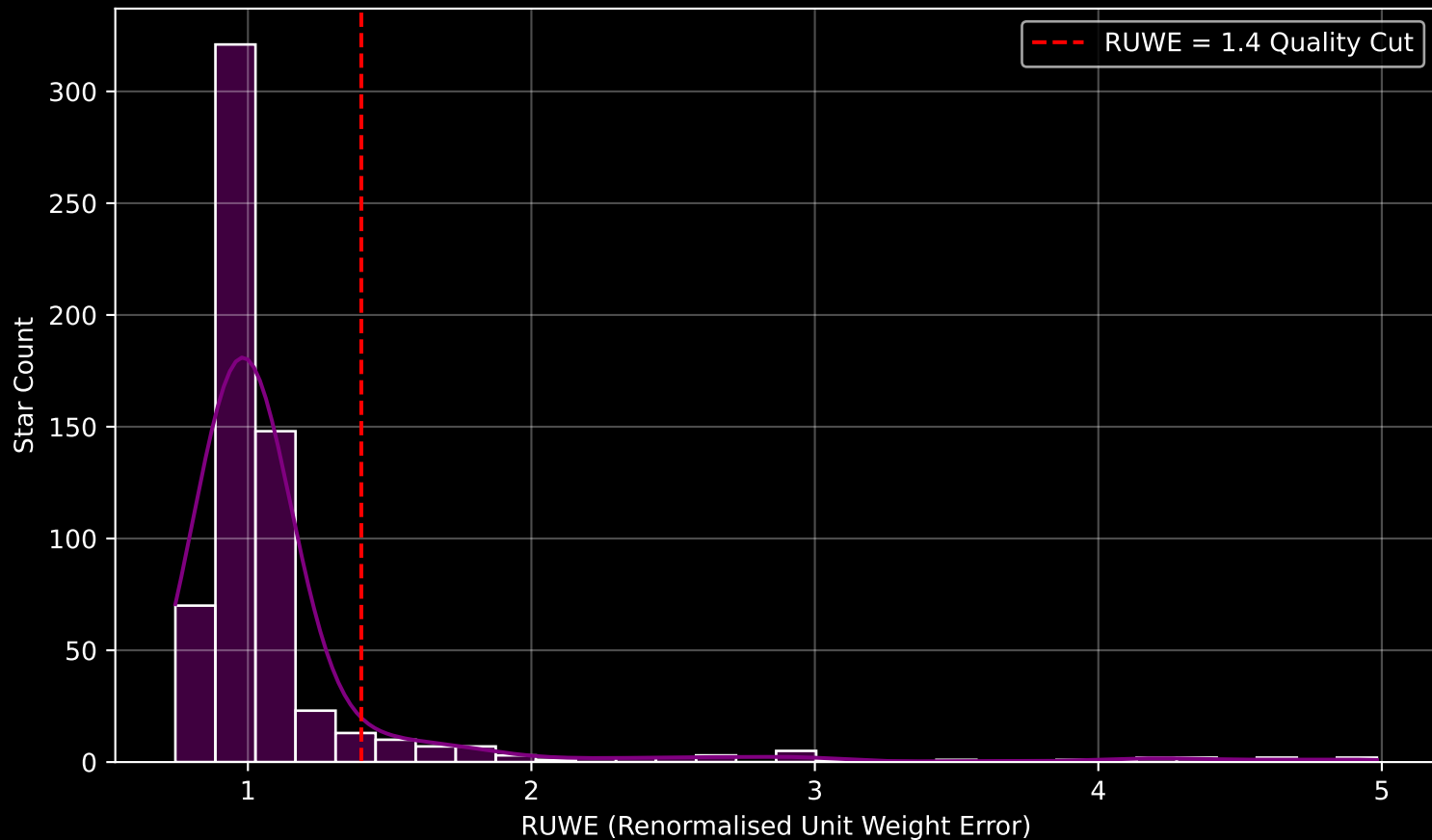
GAPOGEE DR17 Field [K18_070+14] RUWE Distribution (n= 630)
