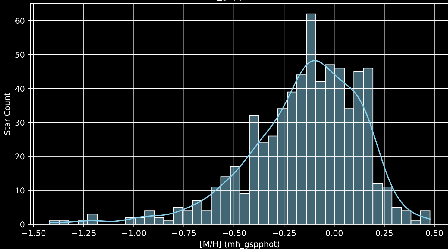
APOGEE DR17 Field: [K18_070+14 [M/H] (mh_gspphot) (n= 646)
