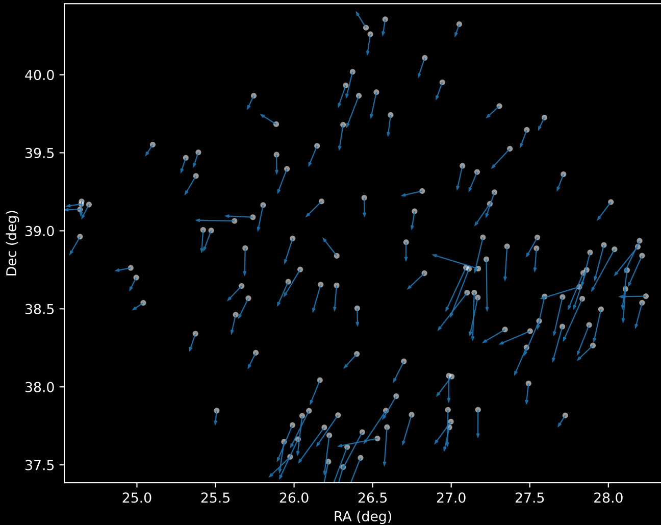
APOGEE DR17 Cluster 20 Proper Motion Vectors (n=129)
