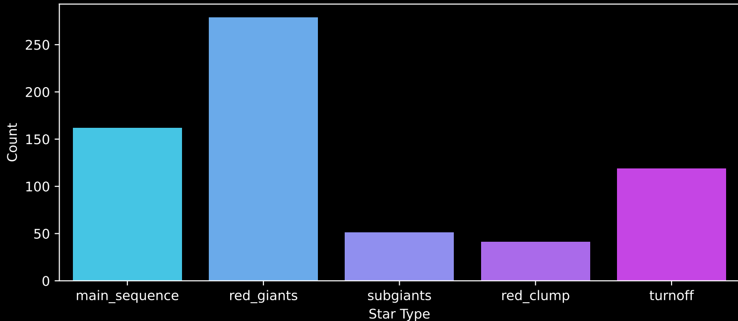
APOGEE DR17 Field: [K18_070+14] Count plot of Star Type
