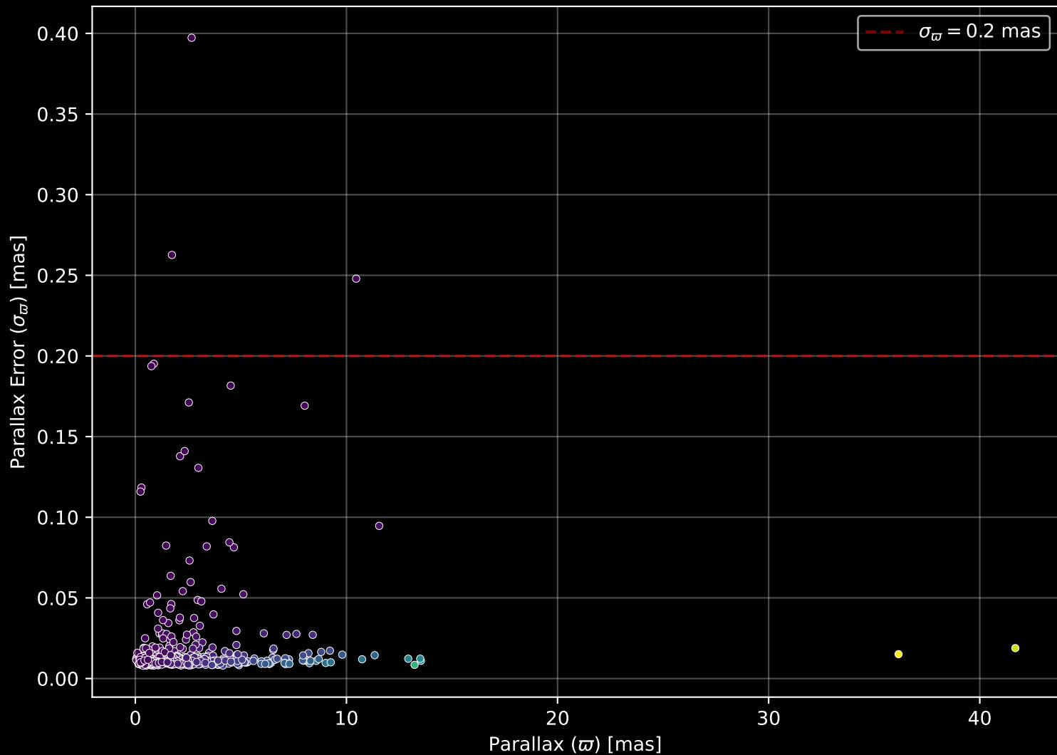
APOGEE DR17 Field: [K18_070+14] Parallax Quality (n= 652)
